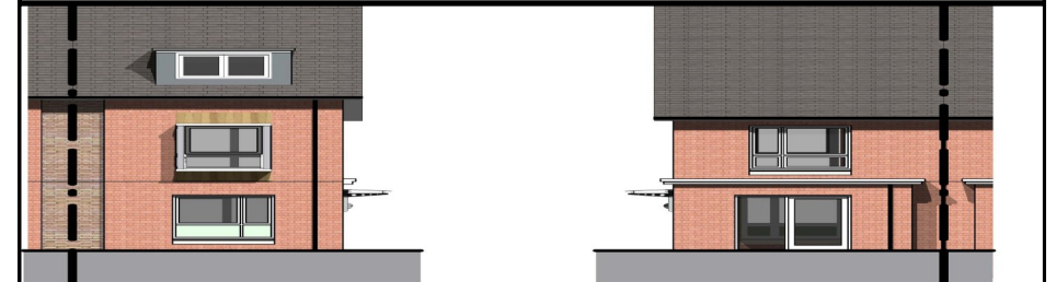
Living room side elevation Kitchen side elevation
